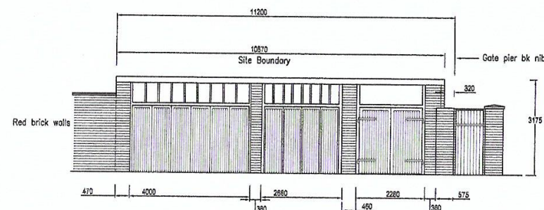
Front Elevation to Lansdowne Place Lane
